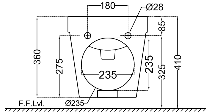
BACK VIEW
