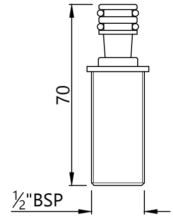
SPOUT NIPPLE
