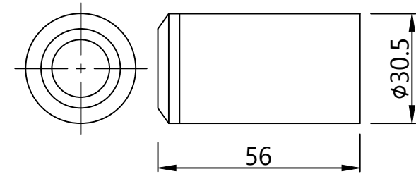
SLEEVE
