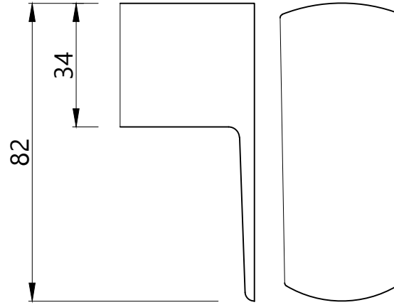
HANDLE
