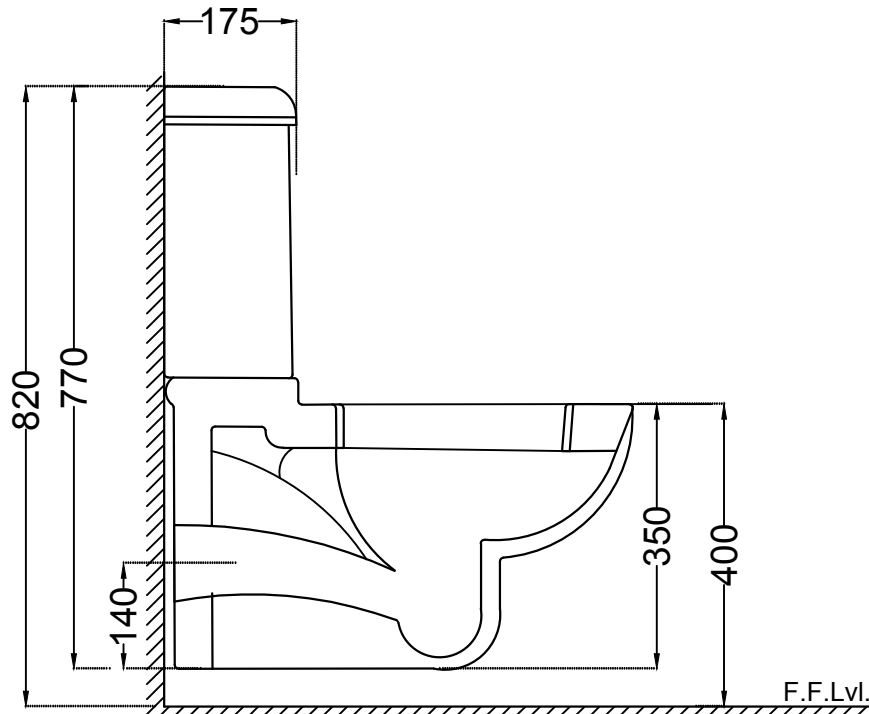
SIDE VIEW
